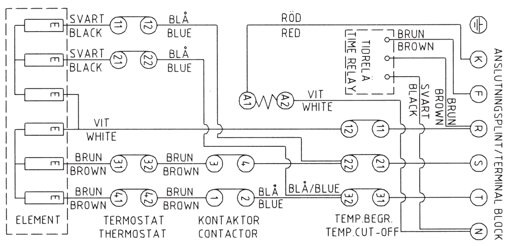
Wiring diagram
